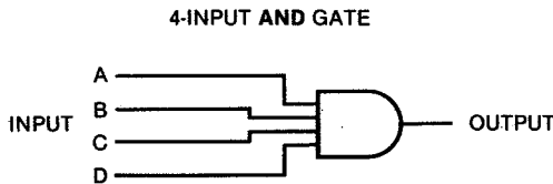
Fig. 1-11. A four-input AND gate.
